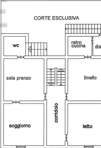
piano terra H 3.00
